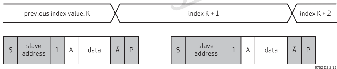
figure 2-15 SCCB single read from current location
