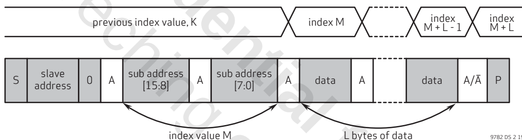
figure 2-19 SCCB sequential write to random location
