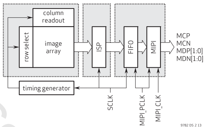
figure 2-12 clock connection diagram
