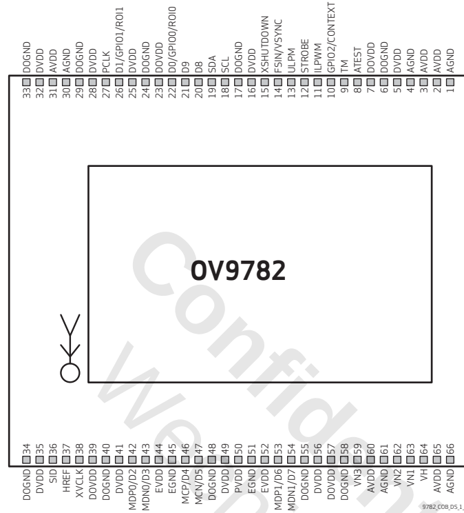
figure 1-1 pad diagram
