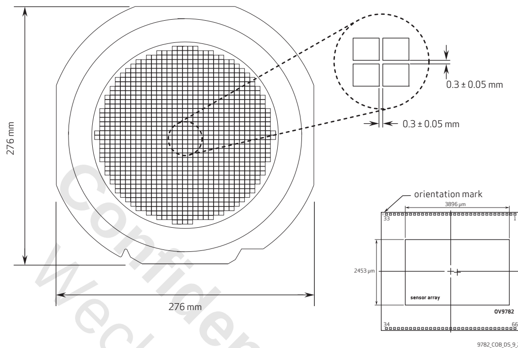
figure 9-2 OV9782 RW physical diagram
