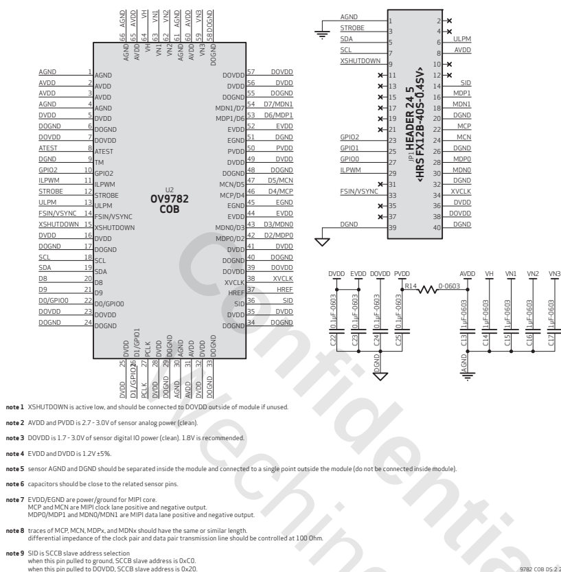
figure 2-2 reference design schematic
