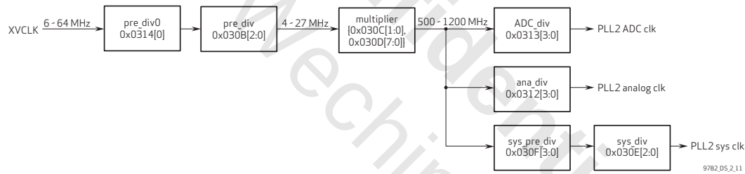
figure 2-11 PLL2 clock diagram
