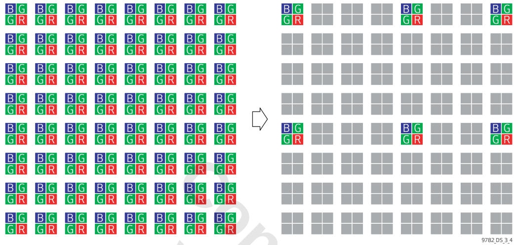
figure 3-4 example of 4:1 skipping
