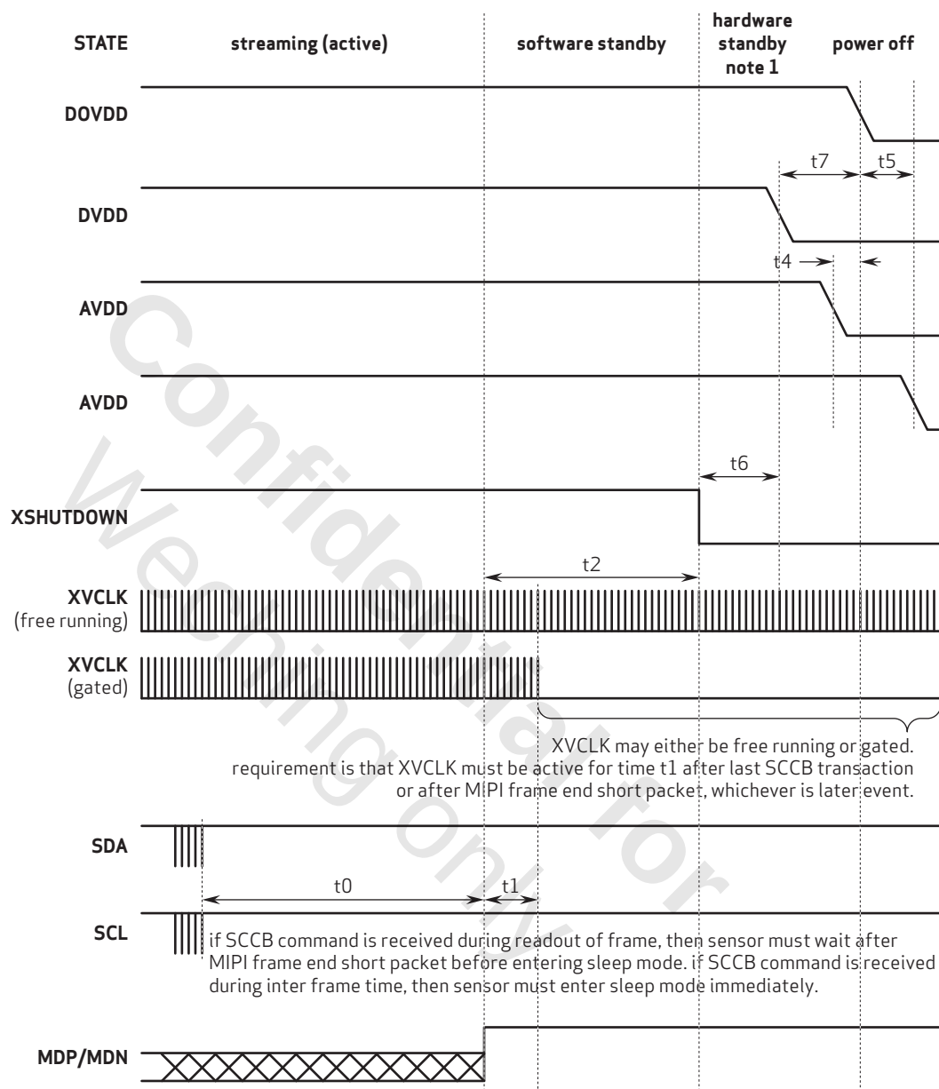
figure 2-8 power down sequence
