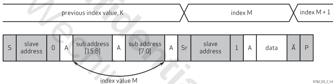
figure 2-14 SCCB single read from random location
