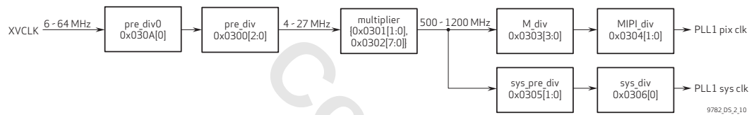
figure 2-10 PLL1 clock diagram
