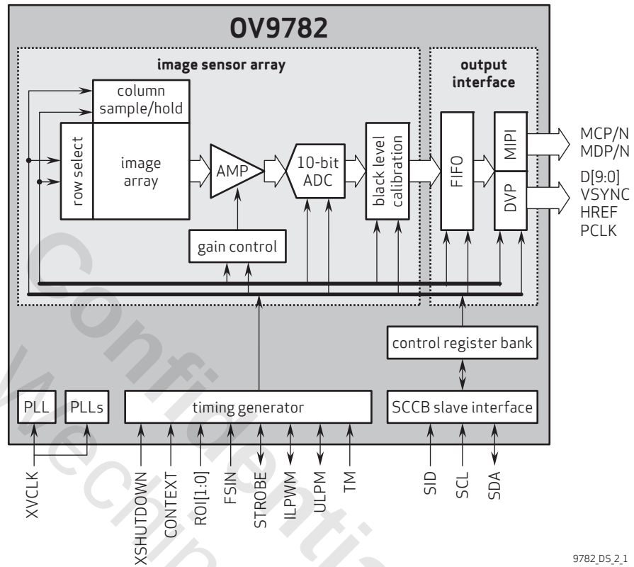
figure 2-1 OV9782 block diagram
