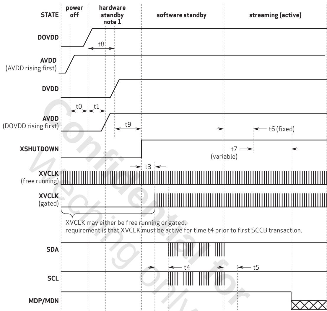
figure 2-7 power up sequence
