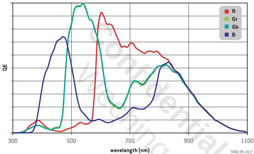
figure 10-3 spectrum response curve
