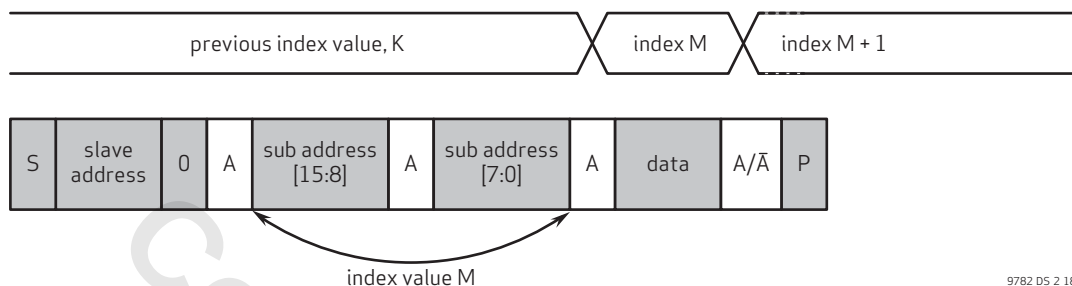
figure 2-18 SCCB single write to random location
