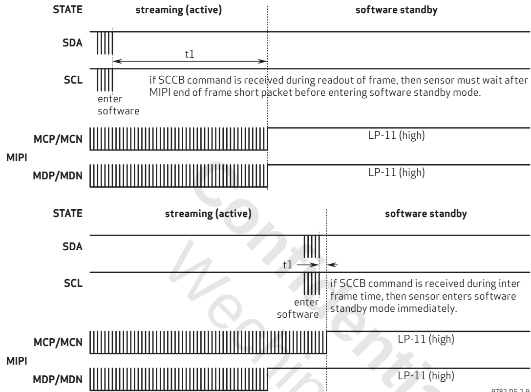
figure 2-9 standby sequence
