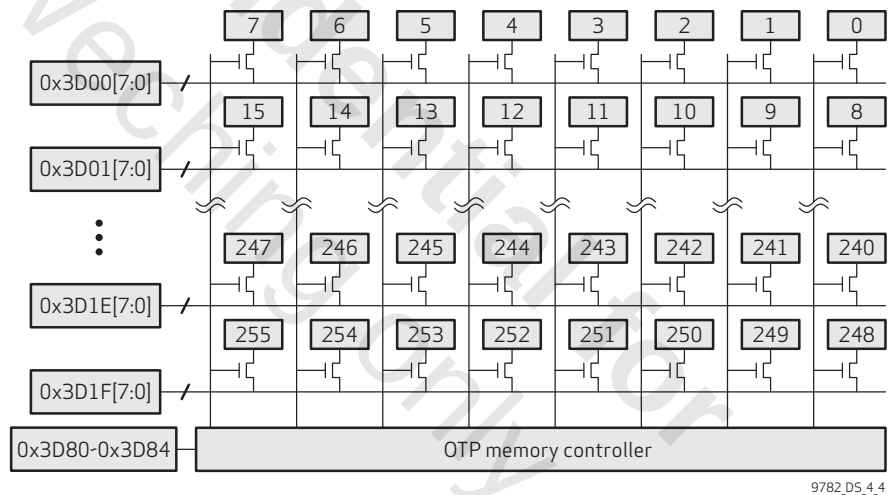
figure 4-4 OTP access
