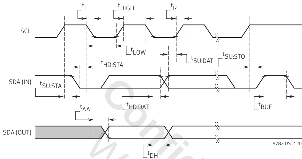
figure 2-20 SCCB interface timing
