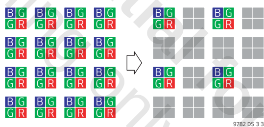
figure 3-3 example of 2:1 skipping
