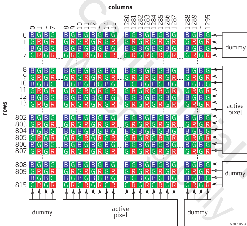
figure 3-1 sensor array region color filter layout
