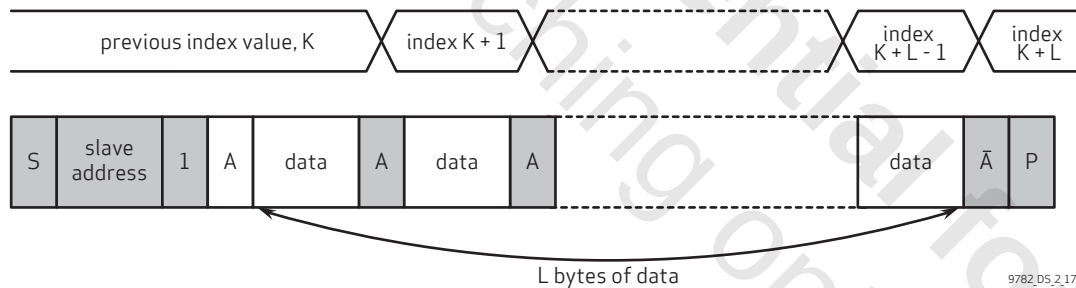
figure 2-17 SCCB sequential read from current location
