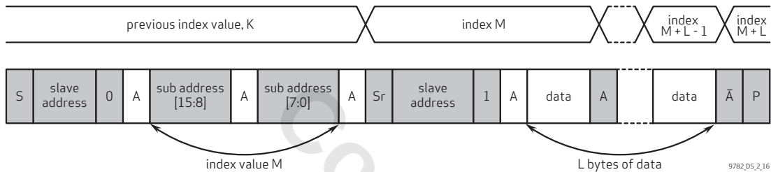
figure 2-16 SCCB sequential read from random location
