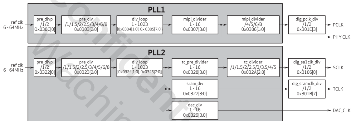
figure 2-6 clock scheme
