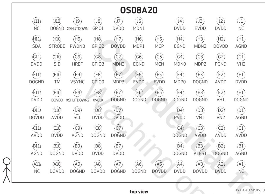
figure 1-1 pin diagram
