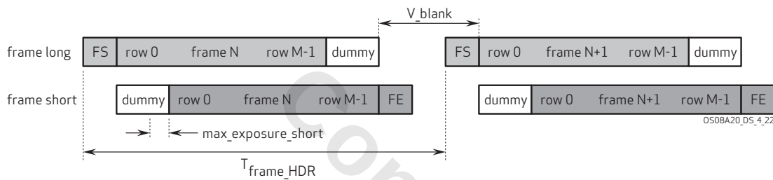
figure 4-22 set staggered HDR with no VC
