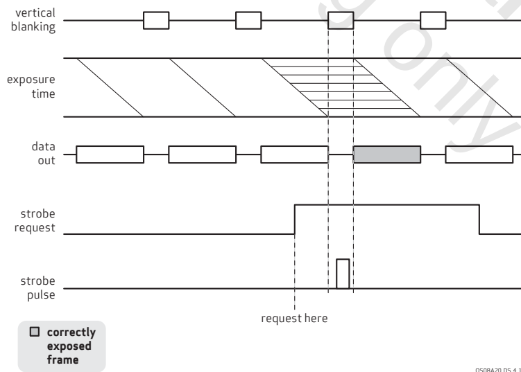
figure 4-13 LED 4 mode
