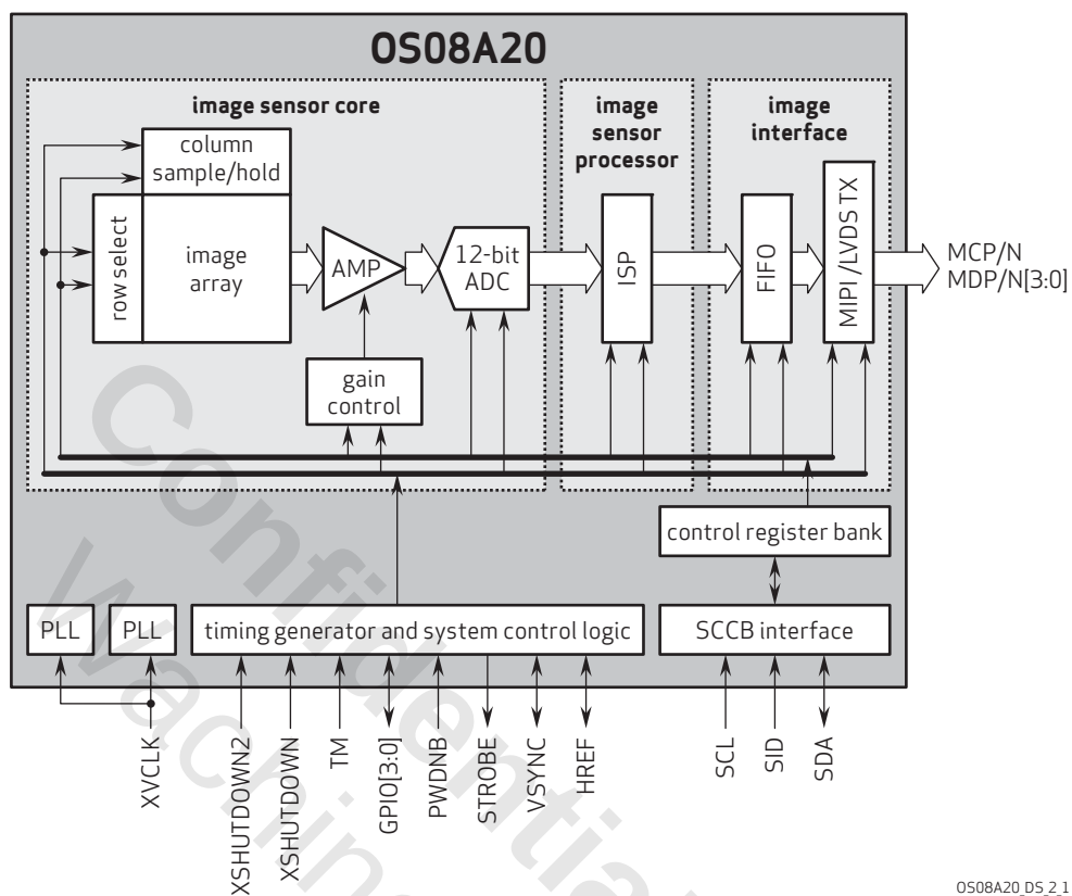
figure 2-1 OS08A20 block diagram
