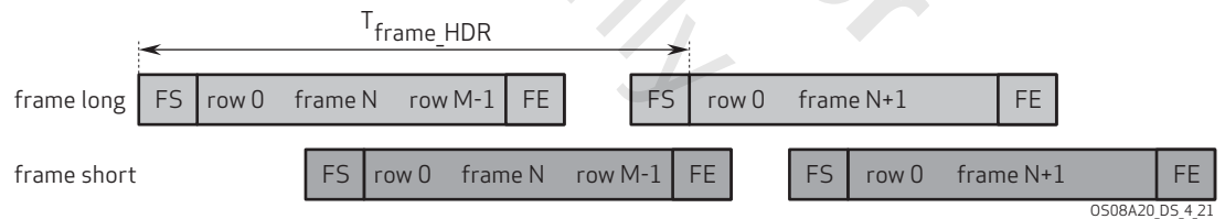
figure 4-21 set staggered HDR
