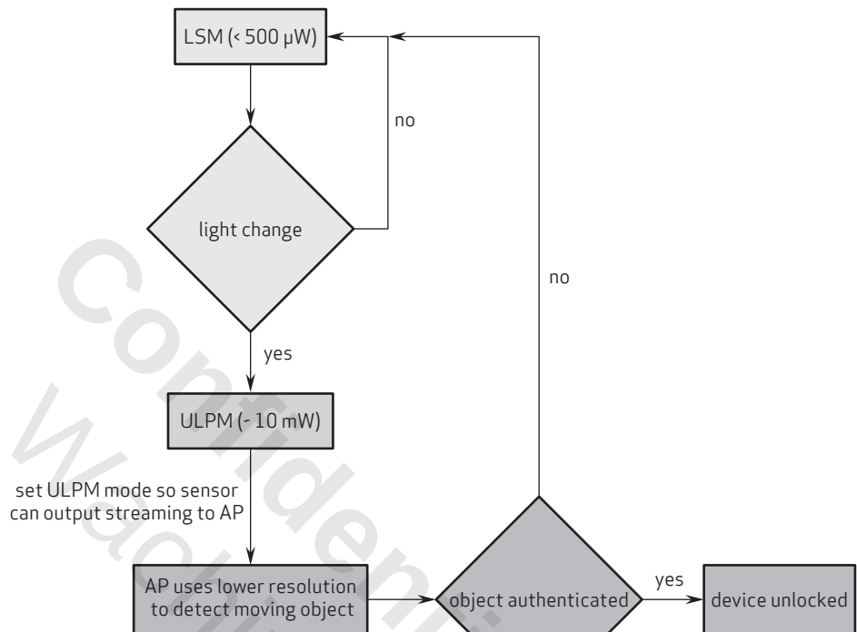
figure 4-14 low power mode example
