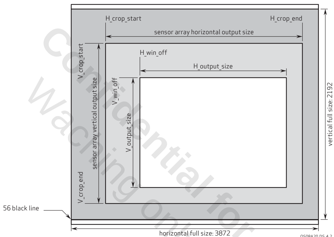
figure 4-2 image windowing
