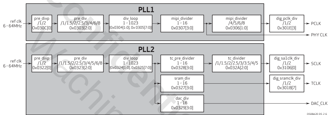
figure 2-6 clock scheme
