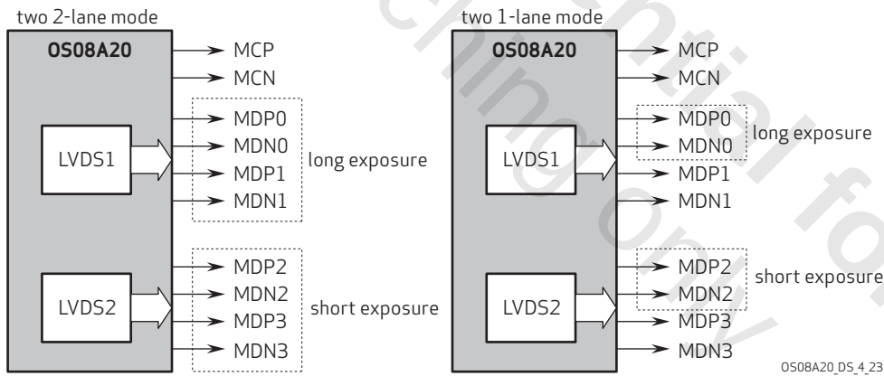
figure 4-23 LVDS axis mode
