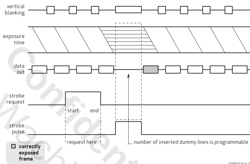
figure 4-11 LED2 mode
