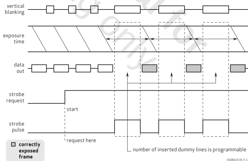
figure 4-11 LED2 mode
