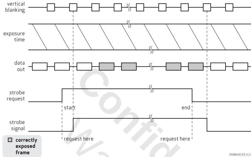
figure 4-12 LED 3 mode
