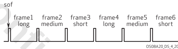
figure 4-20 sequential HDR mode
